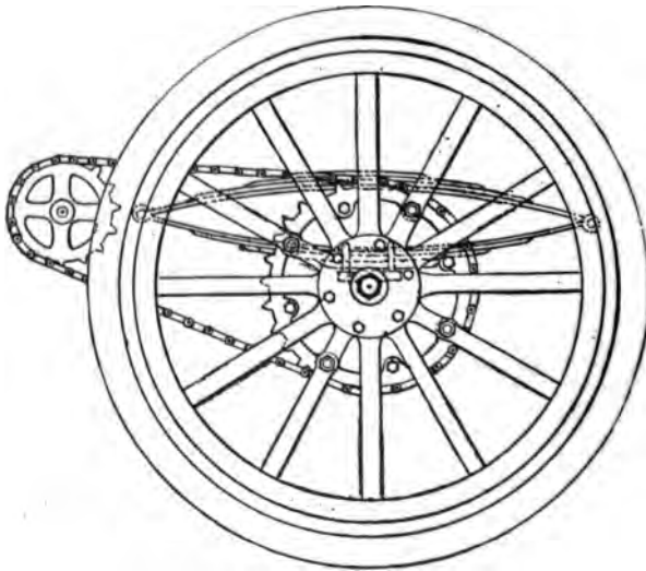
FIG. 18.—Single wheel of a type of car having double-chain drive from a jack-shaft parallel to the dead rear axle
